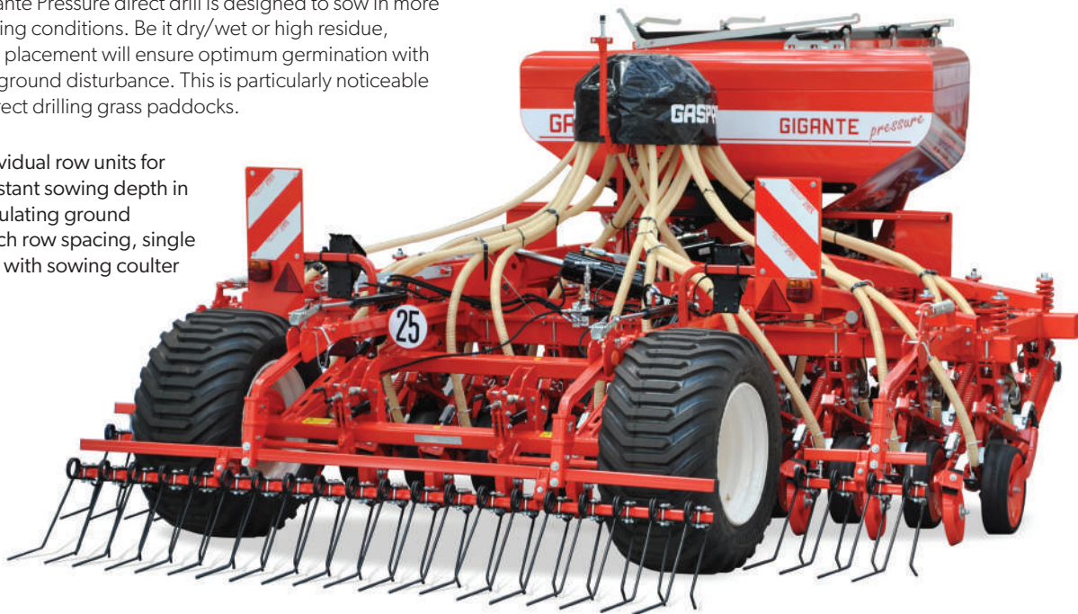
Single shot seed and fertiliser distribution system
